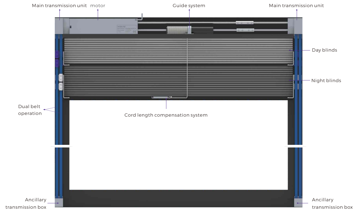
The 3rd generation day and night honeycomb skylight structural diagram
